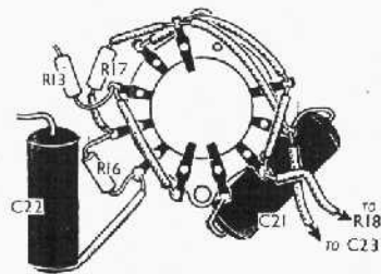
Sketch showing the tone control switch unit assembly as it appears when removed from the chassis. It is drawn as seen from the rear of an inverted chassis.
