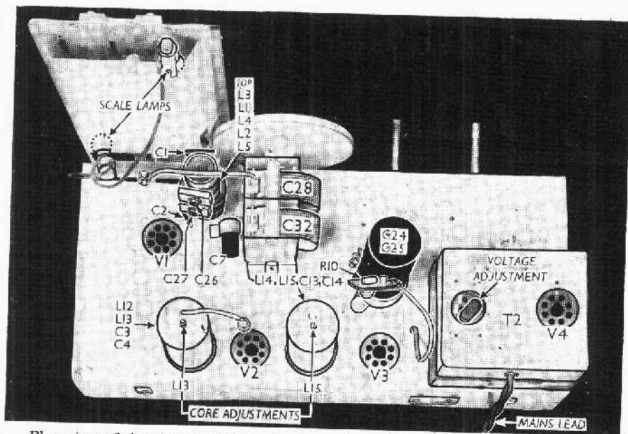
Plan view of the chassis. The mains transformer T2 cover forms a power unit containing the mains lead entry and the rectifying valve V4. R10 is mounted on the top cap connector of V3.
